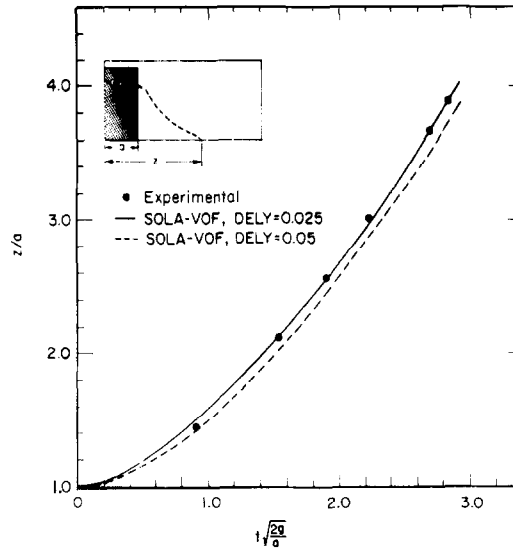
FIG. 7. Comparison of calculated results with experimental data for the broken dam problem.
